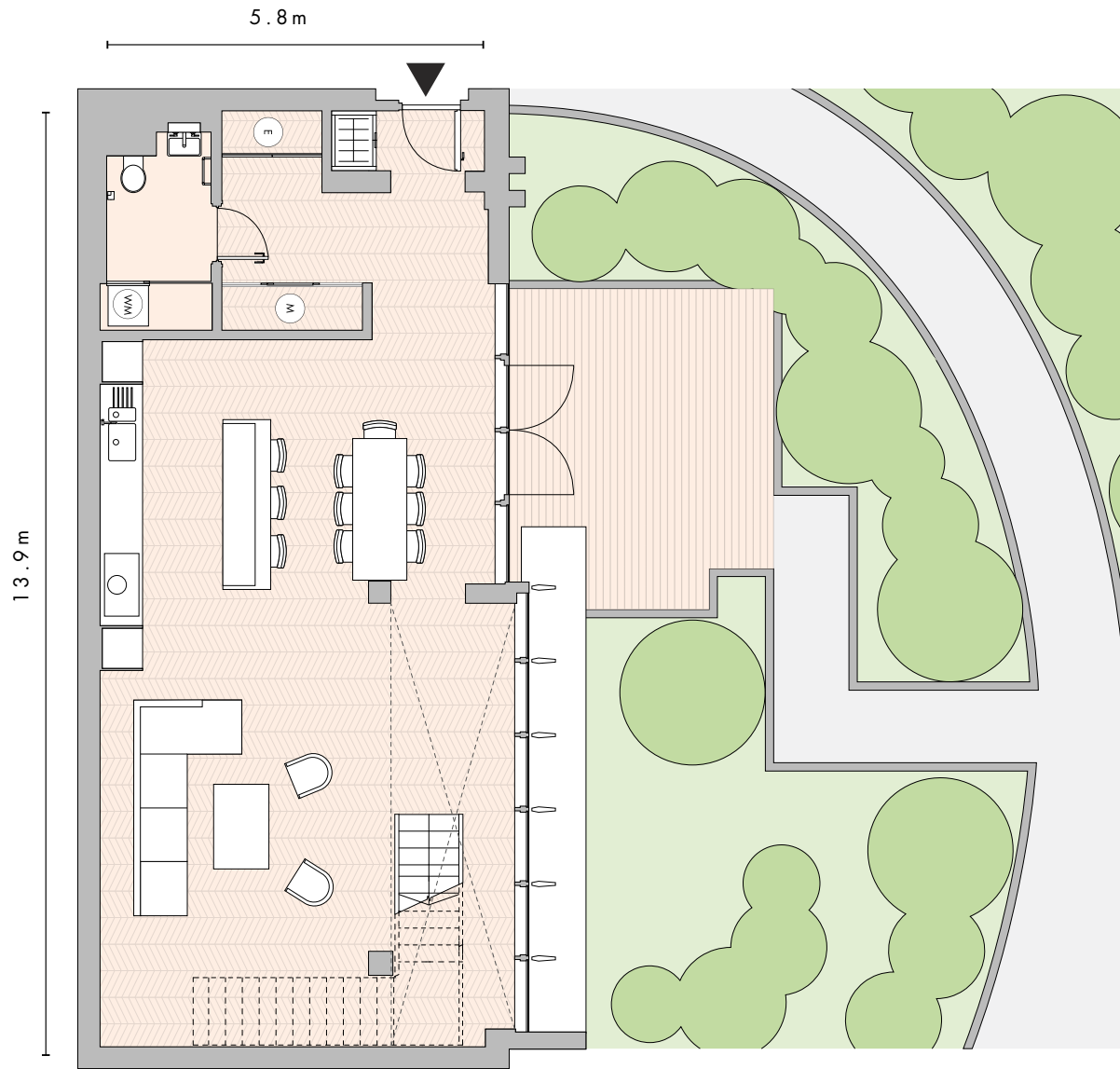
LOWER FLOOR
