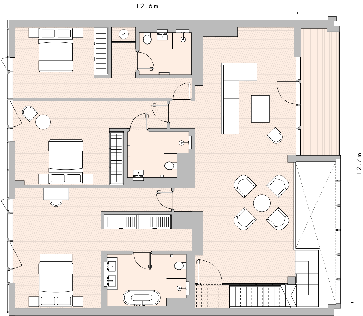
UPPER FLOOR
