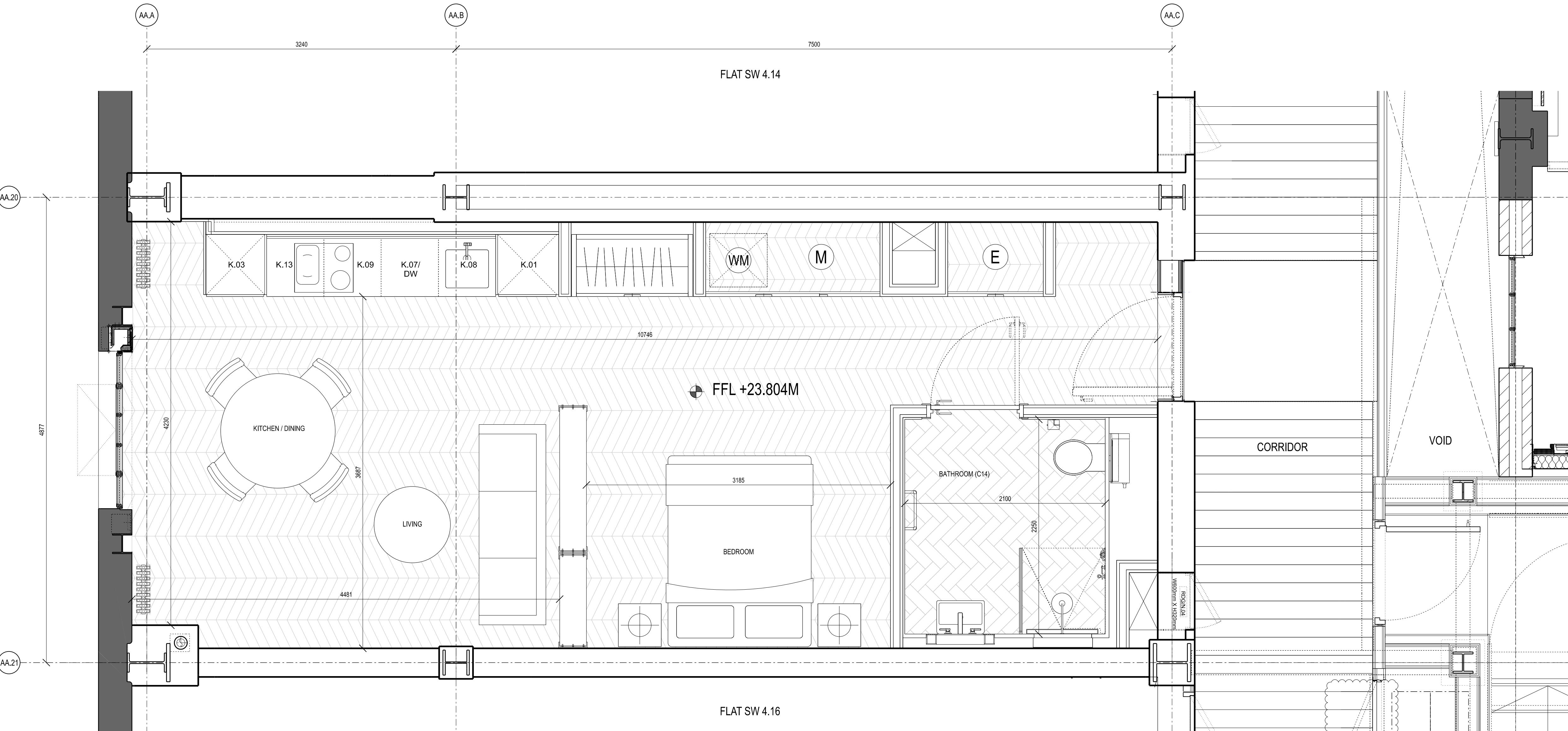
01 FLAT SW 4.15 - GENERAL ARRANGEMENT PLAN - PROPOSED 1:25
