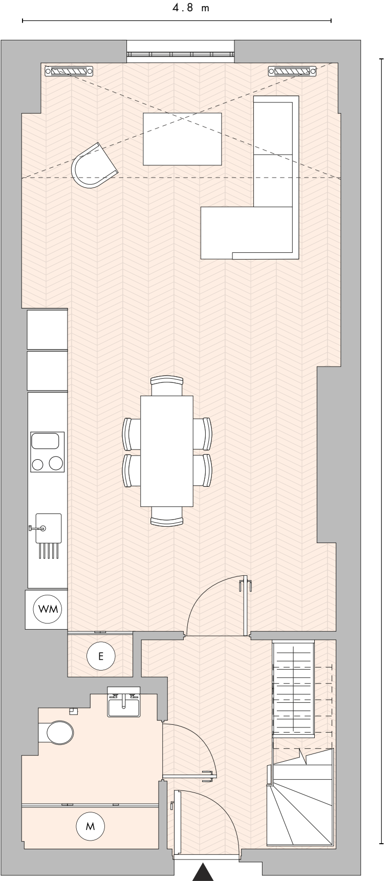
LOWER FLOOR
